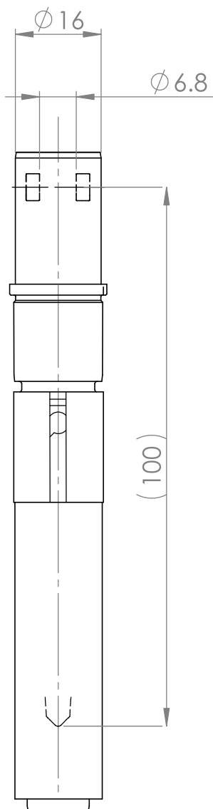
HF100 For speeds up to 25000* rpm
